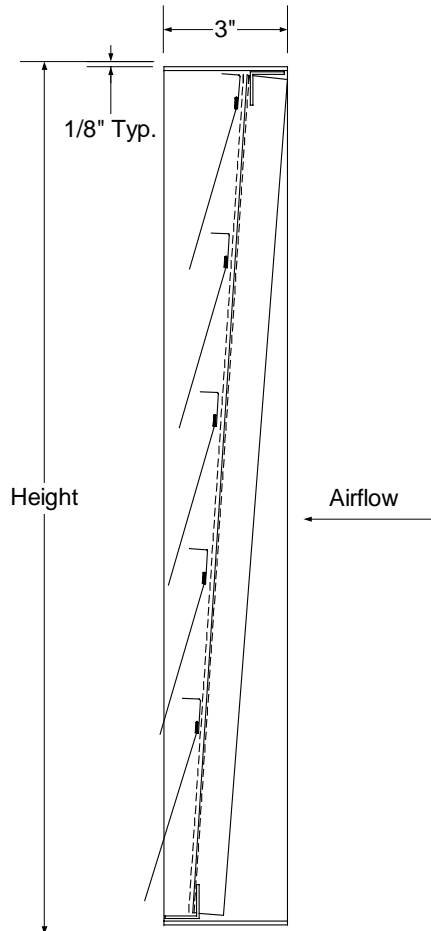
Section View
