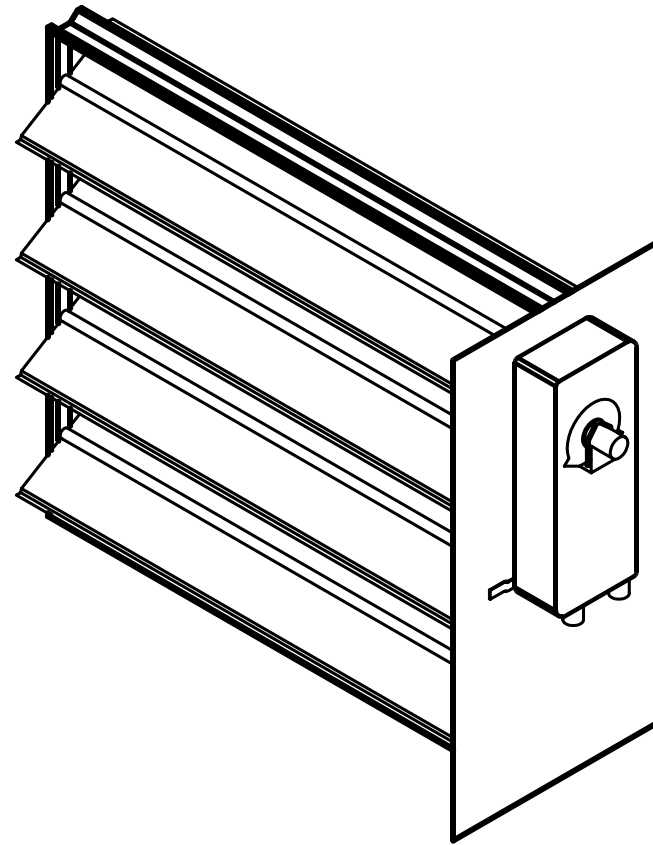
STANDARD MOUNTING ACTUATOR MOUNTED ON FACTORY INSTALLED SIDE PLATE EXTERNAL TO DUCT
